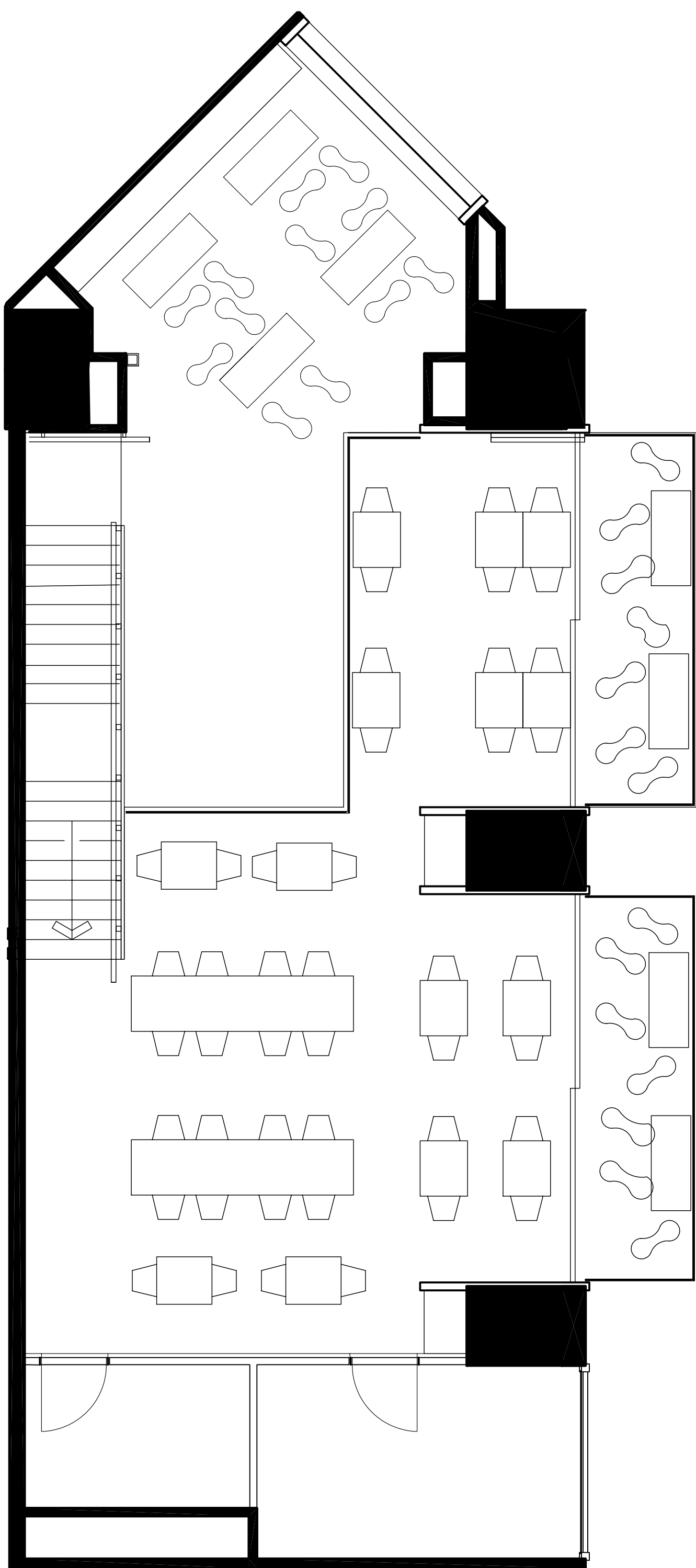
Spiga - level one
